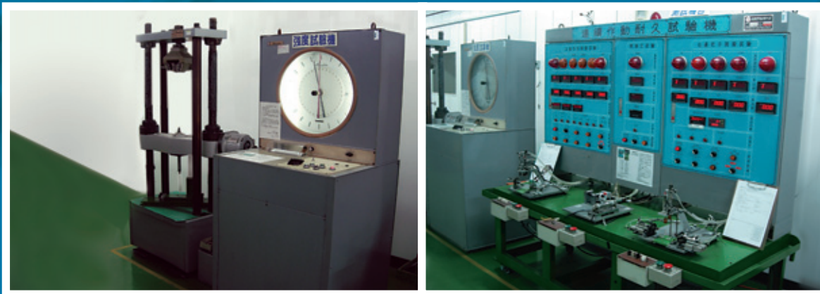
4. 強度拉力測試機台 Strength of tensile force tester
